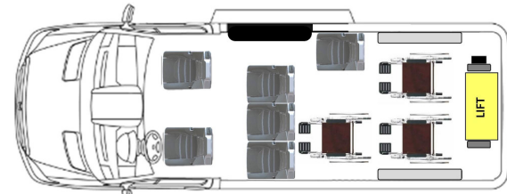
LWB Rear Lift 6 Passenger + 3 WC
