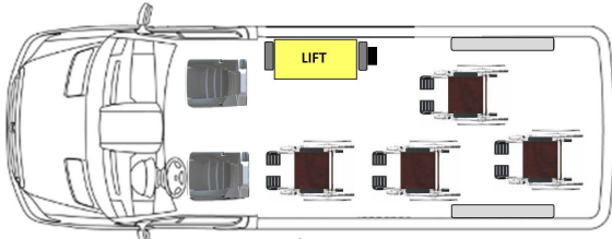
LWB Side Lift 2 Passenger + 4 WC
