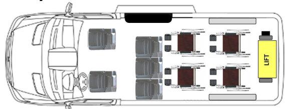
LWB Rear Lift 5 Passenger + 4 WC
